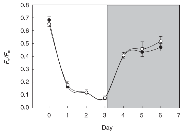
Fig. 7 Recovery of maximum PSII efficiency ( F_v/F_m ) for pretreated red (open symbols) and green (closed symbols) Galax urceolata leaves. Light was shone on acyanic abaxial surfaces only. White area, high-stress treatment; gray area, recovery period. Points depicted are means \pm SE of five replicates.
