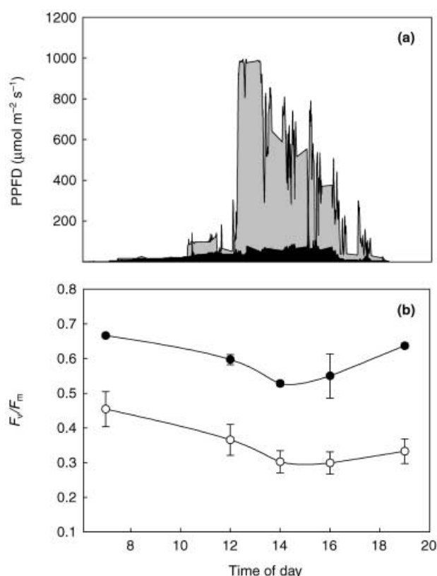
Fig. 1 Typical diel pattern for (a) PPFD; (b) ratio of variable to maximum fluorescence (maximum PSII efficiency, F_v/F_m ) of red (light shading or open symbol) and green (dark shading or closed symbol) Galax urceolata leaves in the field (taken 3 March 2004).
