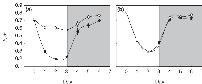
Fig. 8 Recovery of maximum PSII efficiency ( F_v/F_m ) for pretreated red (open symbols) and green (closed symbols) Galax urceolata leaves to high-stress period consisting of (a) green light; (b) red light. Light was shone on adaxial surfaces only. White area, high-stress period, gray area, recovery period. Points depicted are means \pm SE of five replicates.
